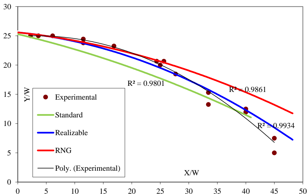
Figure 22. Comparison between numerical simulation and experimental data to prediction about jet center line in different states of k-ε model
