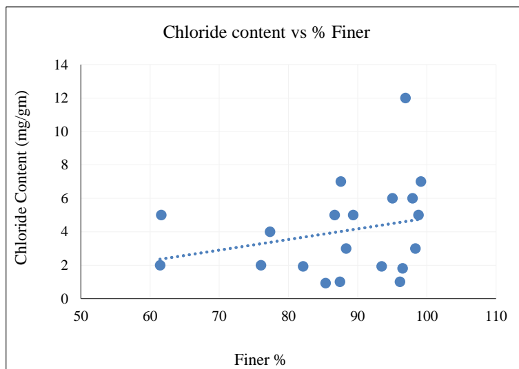
Figure 21. Relationship of Chloride Content with % Finer
