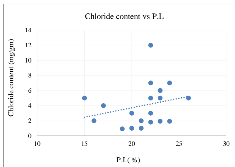
Figure 19. Relationship of Chloride Content with Plastic limit
