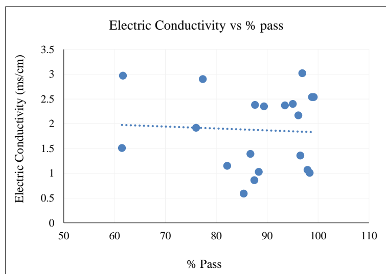
Figure 17. Relationship of Electric Conductivity with % Finer
