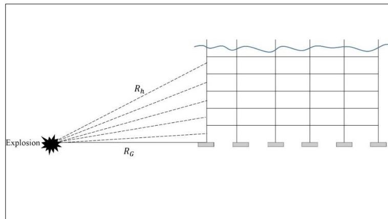
Figure 5. Geometry of building frame for calculating R h
